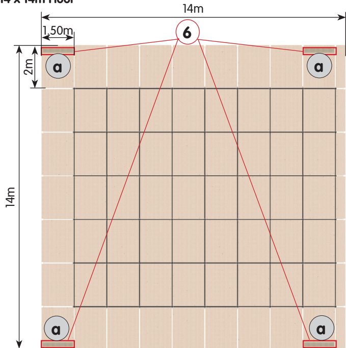
Figures 3 & 4 - Installing the foam area
