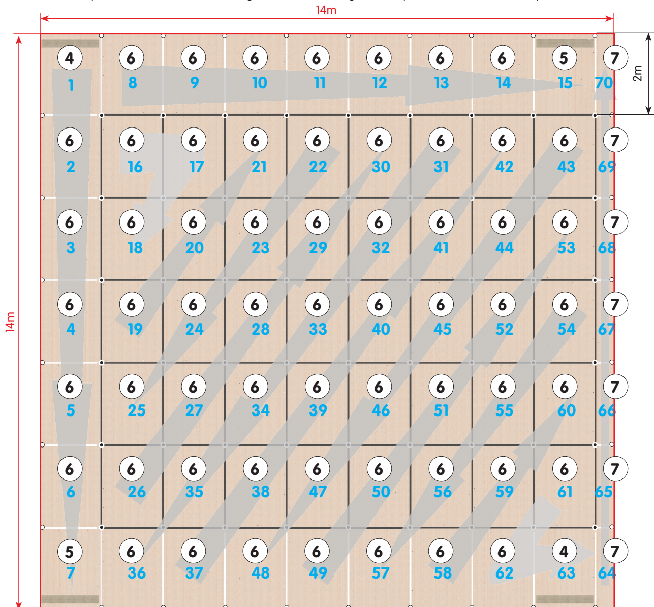
Figure 3 - Arrangement and order of the panels assembly
